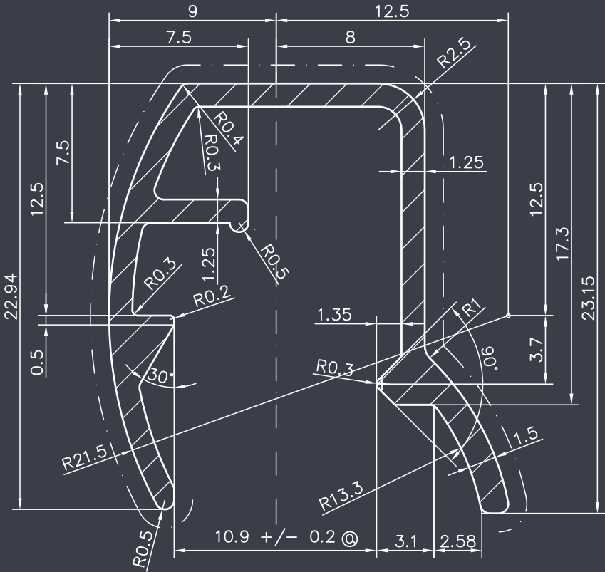
Precision down to the finest detail: cross-section of the aluminium profile for the whiteboard MAULpro
