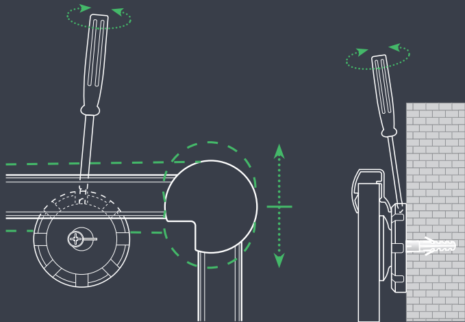
Easy mounting: the MAULpro board can be adjusted easily by up to 6 mm after hanging with the help of the patented MAUL excenter fitting.
